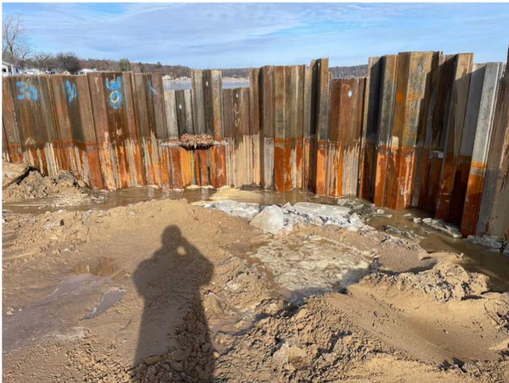
Photo #3: Dewatering progress in the inlet area - Nov 28, 2023, 11:57 AM
